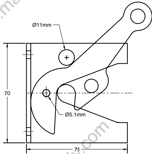
① SELF LOCK GATE LATCH H/D 3 INCH
